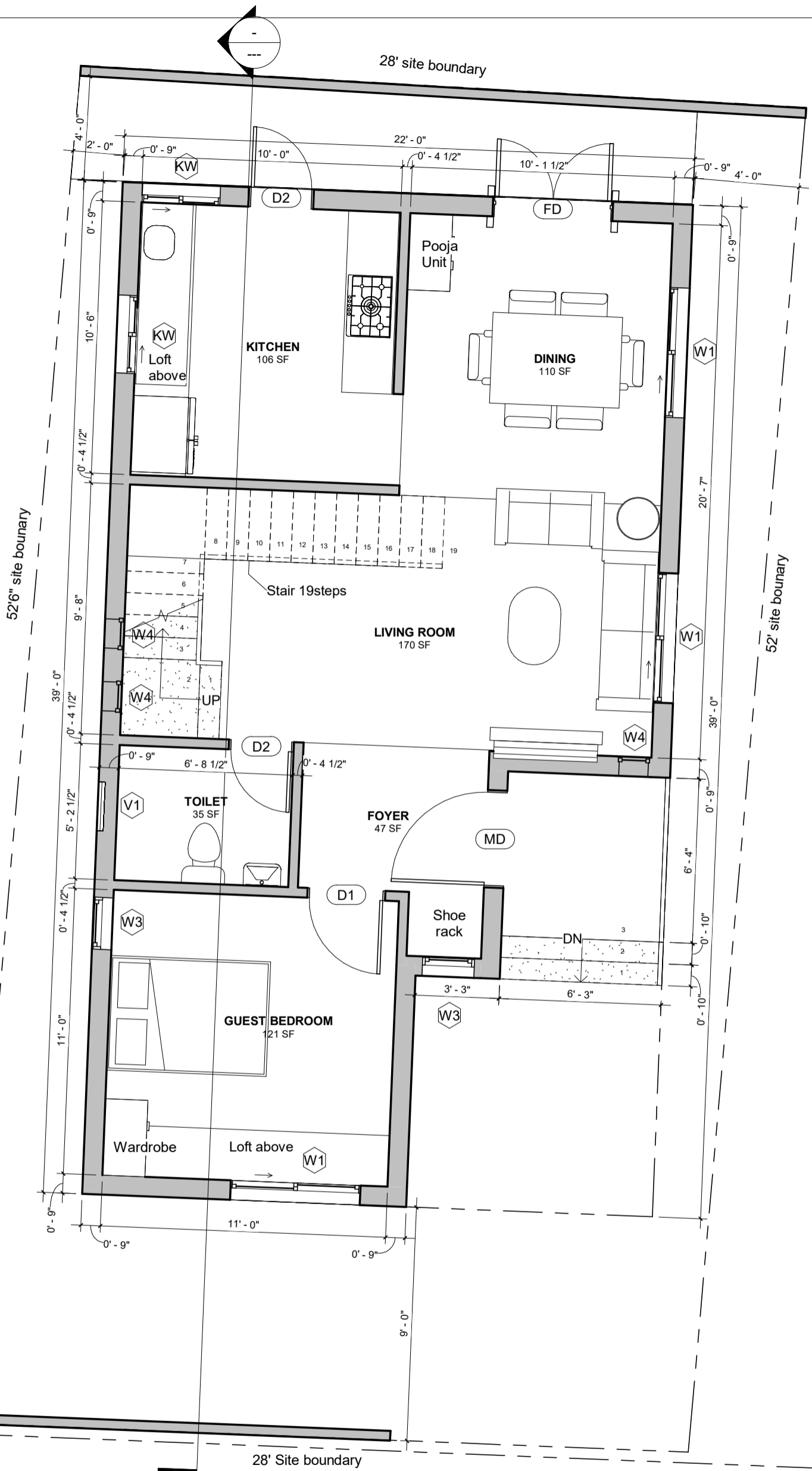
1 Ground Floor Level 1/4" = 1'-0"
